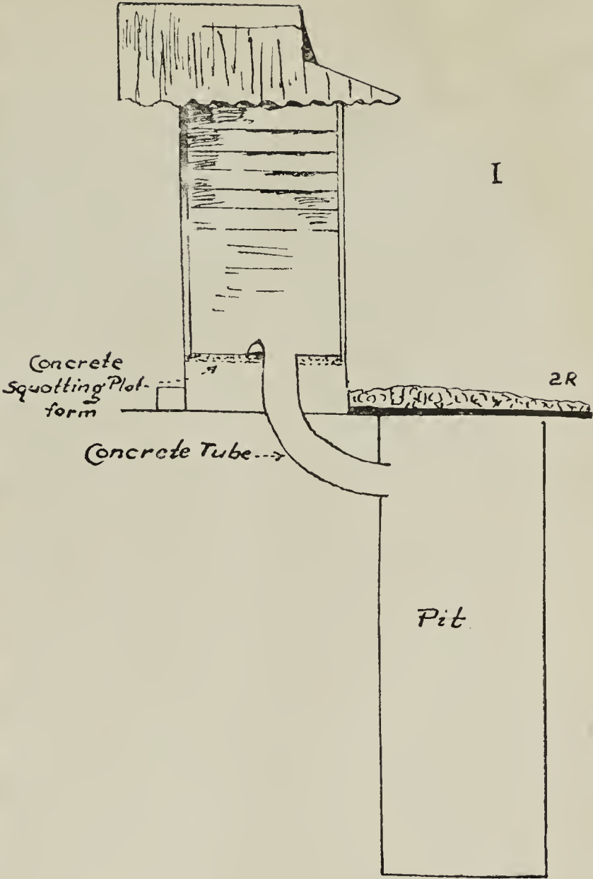
Diagram showing the construction of Latrine I.
